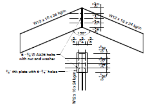
Detail 8
