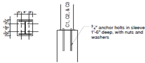
Detail 1
