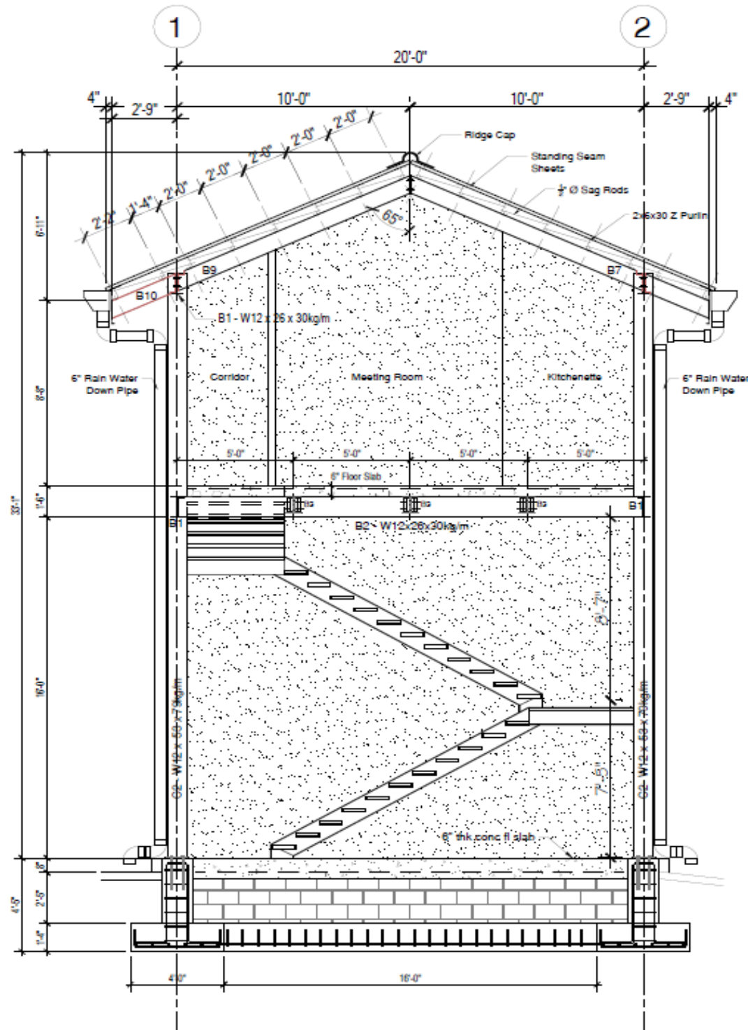
Section B-B
