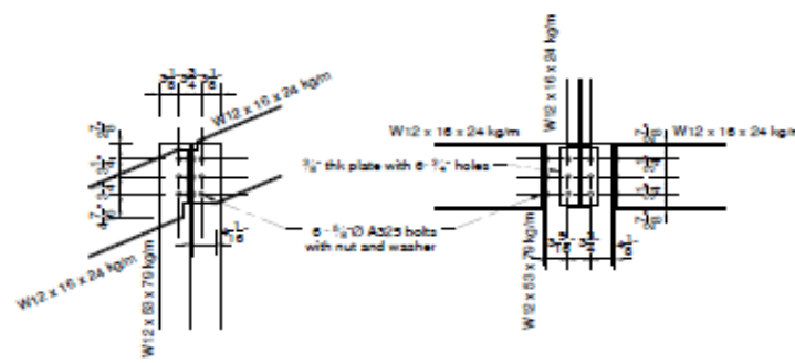
Detail 7
