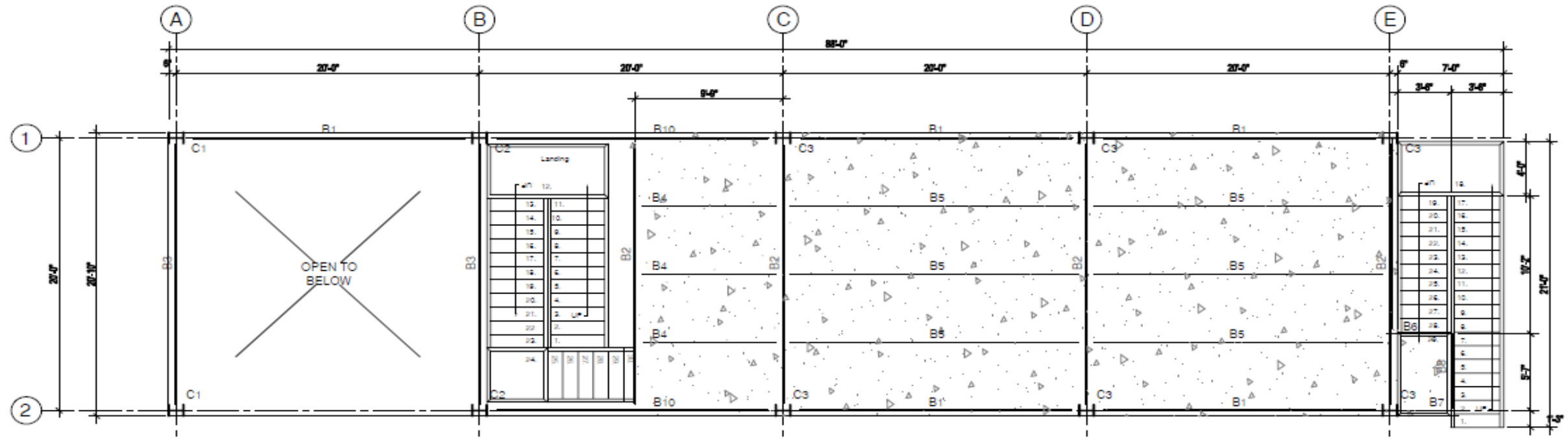
Mezz. Plan
