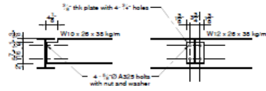
Detail 5
