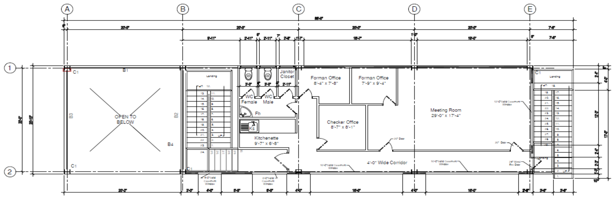
1st Floor Mezz. Plan
