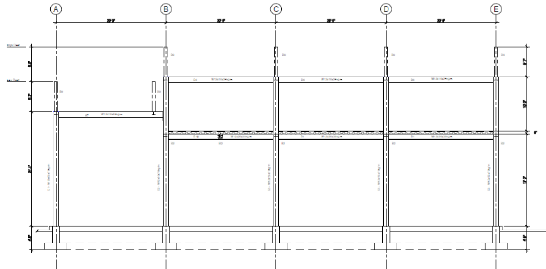
Grid Line 1 & 2
