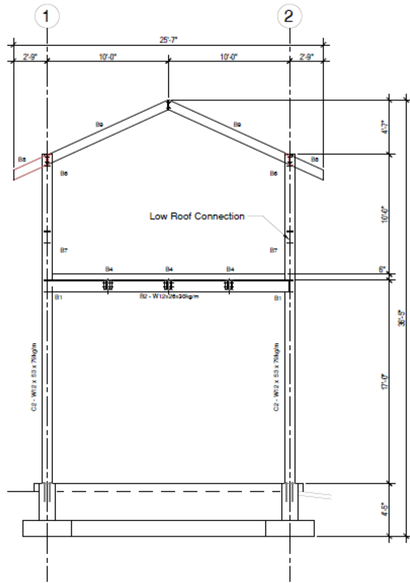
Grid Line B
