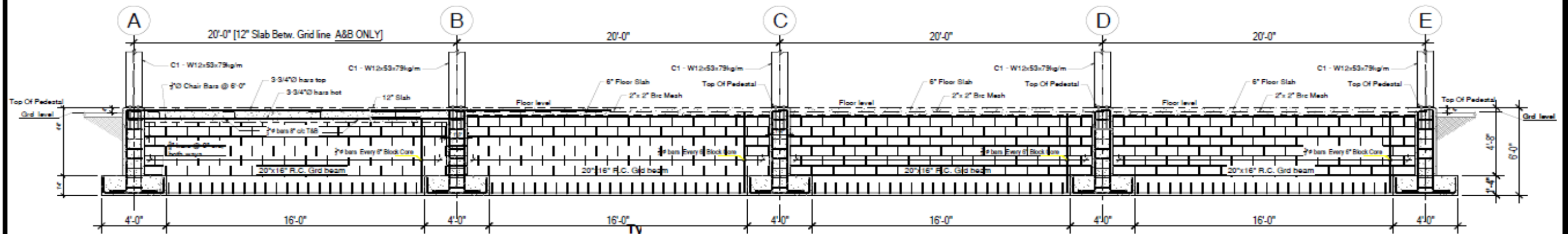
Typical Beam Detail Along Gridline 1&2
