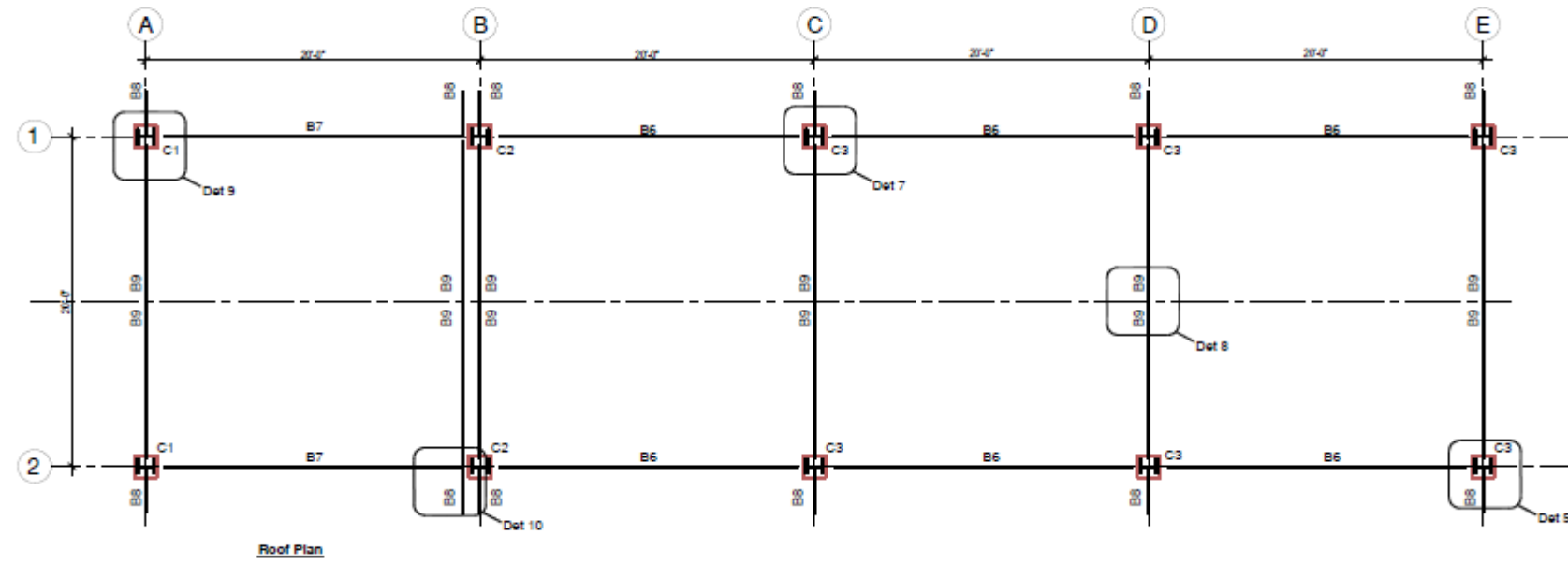
Roof Plan
