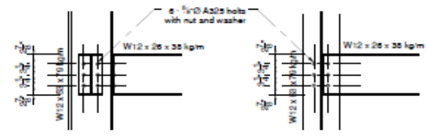
Detail 3
