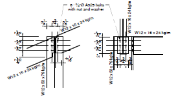
Detail 9
