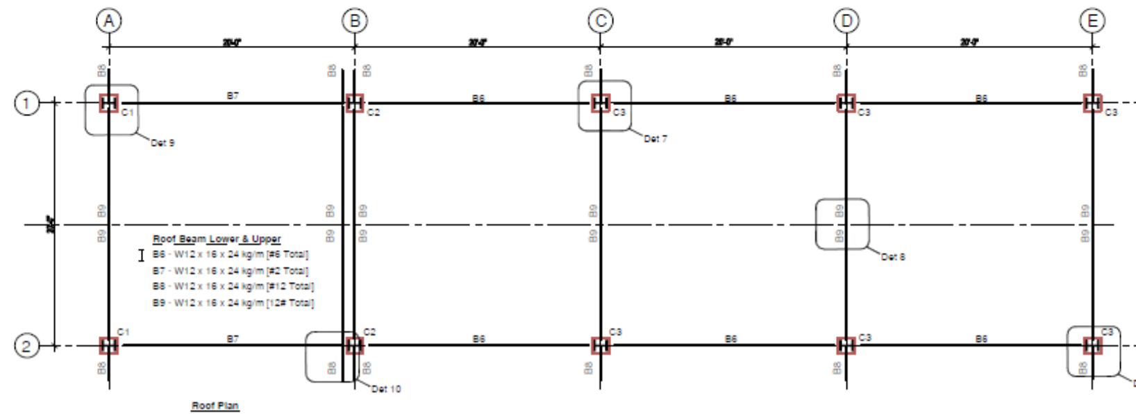
Roof Plan
