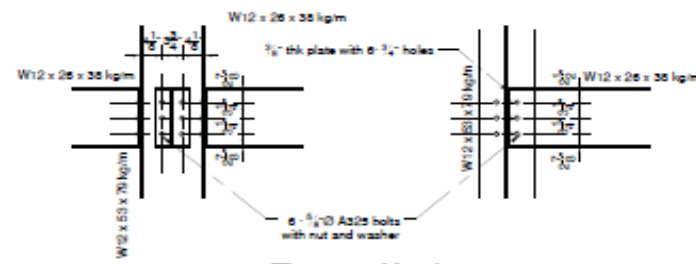
Detail 4
