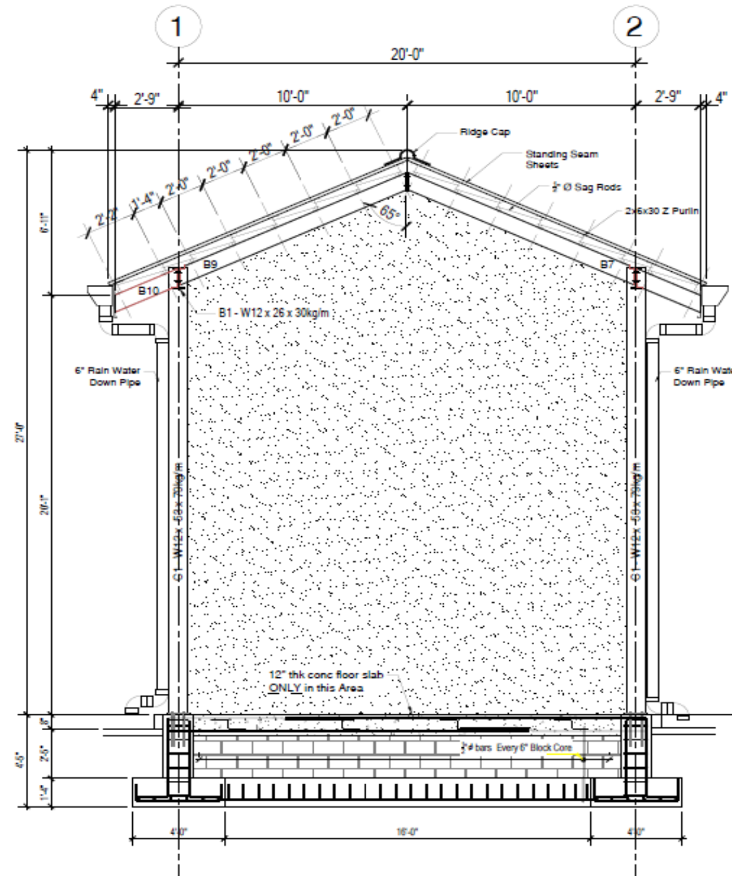
Section B-B
