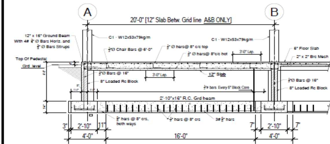
Section 1-1
