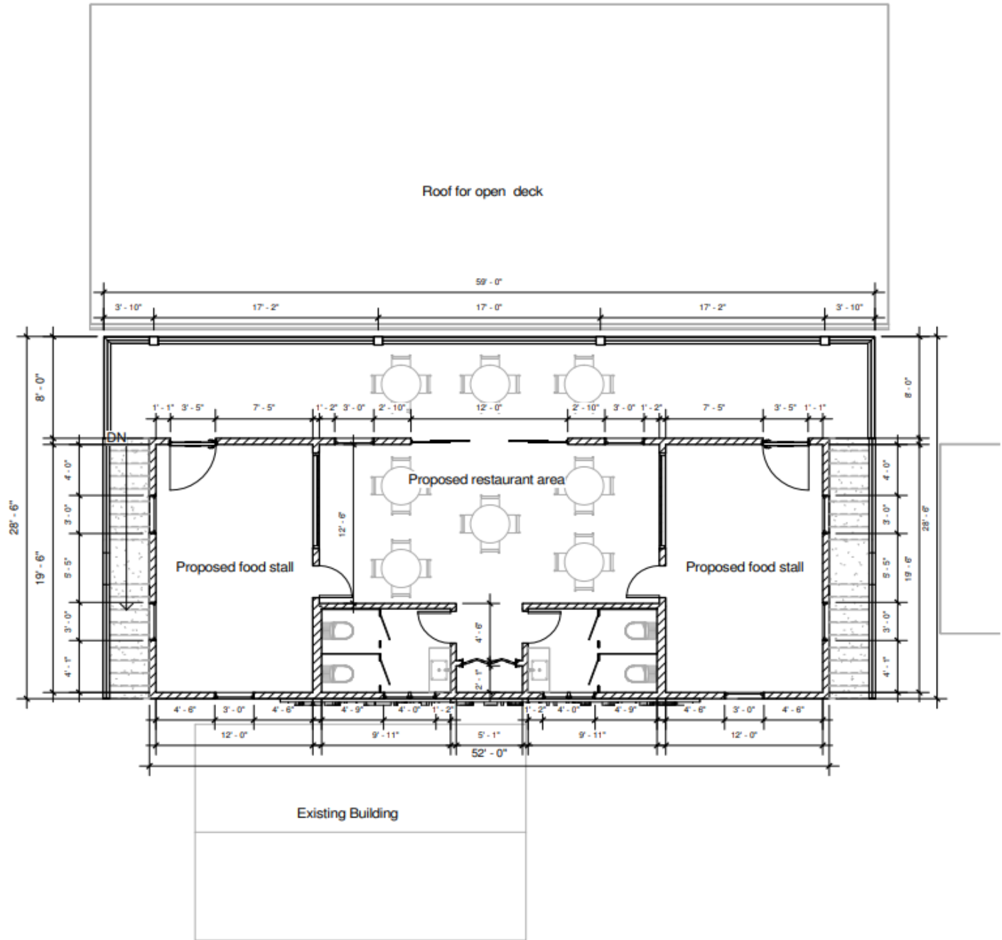
① FIRST FLOOR 1/8" = 1'-0"
