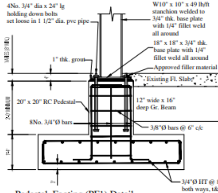
Pedestal, Footing (PF1) Detail SCALE: 1" = 1'-0"
