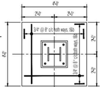
Pad Footing Detail (PF1) SCALE: 1" = 1'-0"
