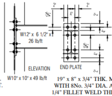
W12" x 6 1/2" x 26 lb/ft Beam Connection To W10" x 10" x 49 lb/ft Stanchion (WEB) SCALE: 1 1/2" = 1'-0"
