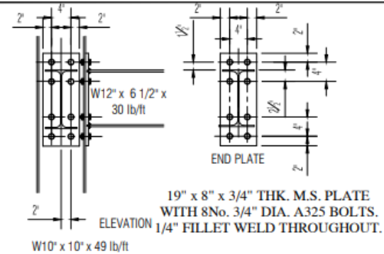
W12" x 6 1/2" x 30 lb/ft Beam Connection To W10" x 10" x 49 lb/ft Stanchion (FLANGE) SCALE: 1 1/2" = 1'-0"
