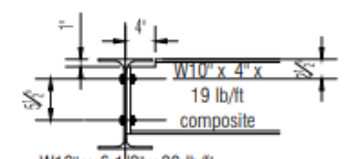
W12" x 6 1/2" x 30 lb/ft Beam Connection To W10" x 4" x 19 lb/ft composite Beam (WEB) SCALE: 1 1/2" = 1'-0"
