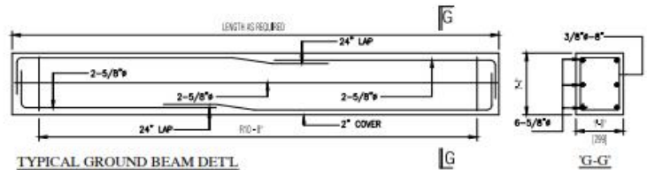
TYPICAL GROUND BEAM DETL
