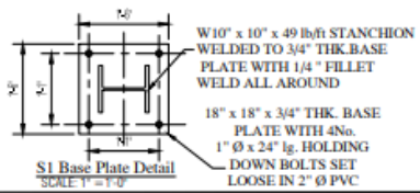
S1 Base Plate Detail SCALE: 1" = 1'-0"
