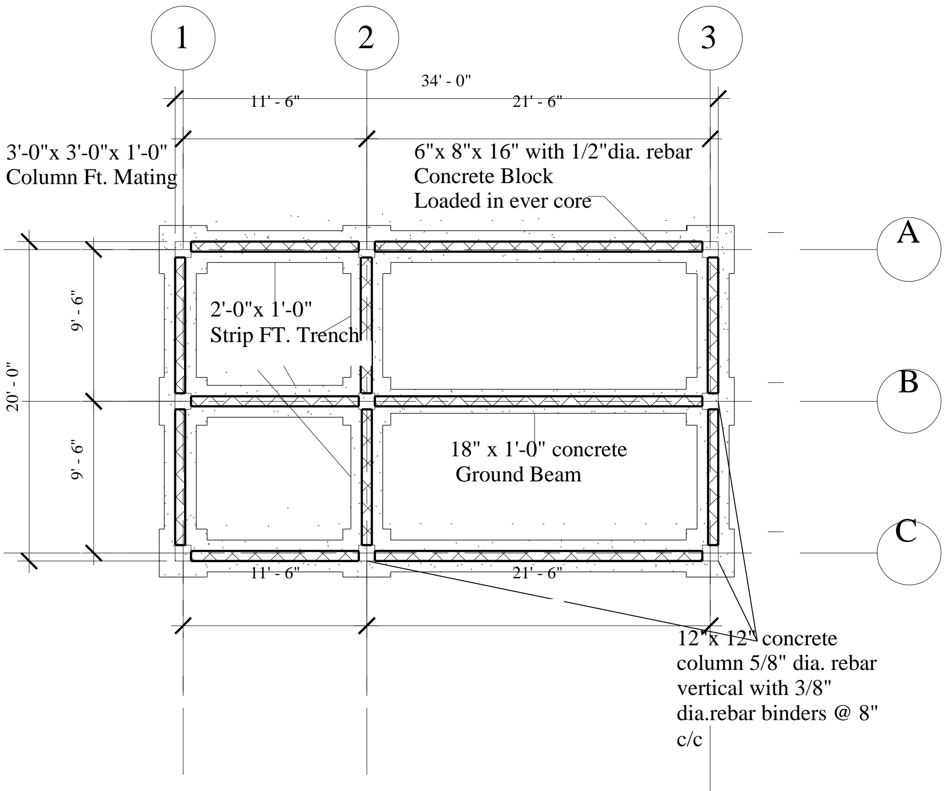
Foundation Plan
