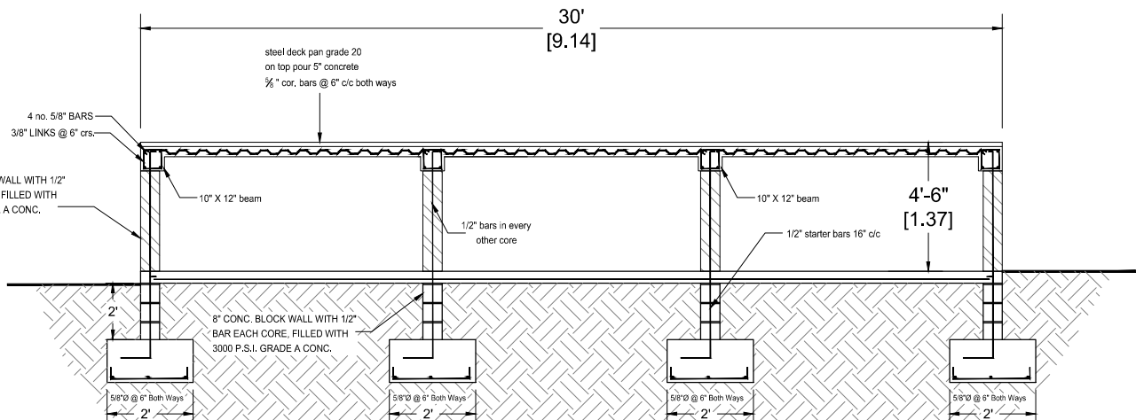
SECTION
