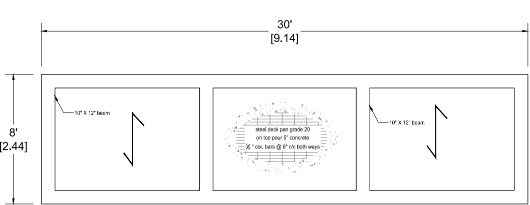
BEAM PLAN
