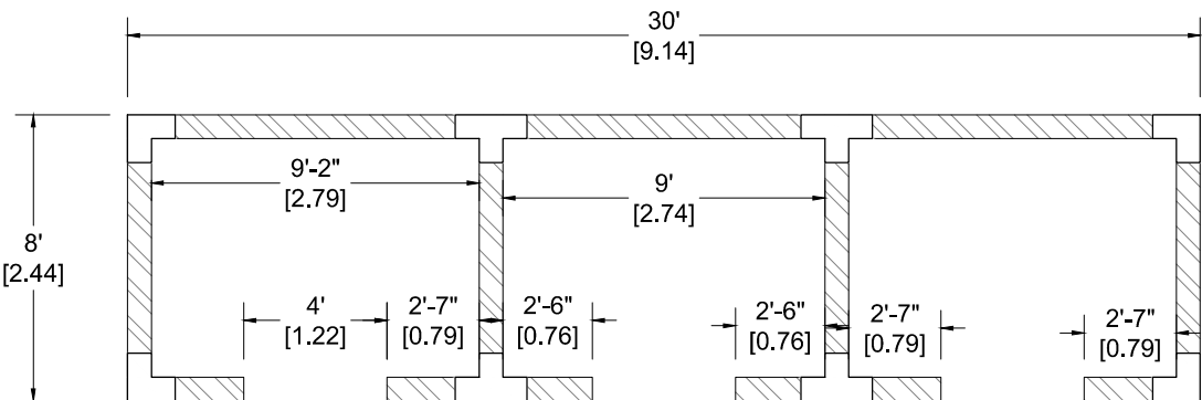
FLOOR PLAN
