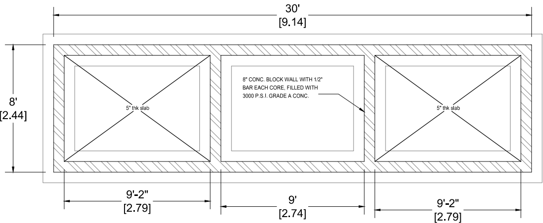
FOUNDATION
