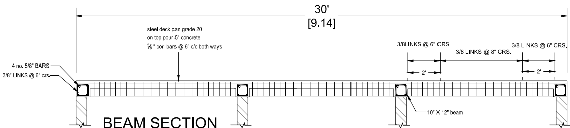
BEAM SECTION
